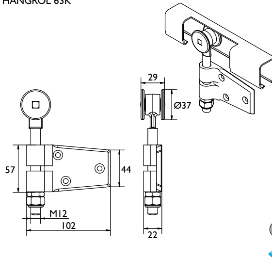
HANGROL 63K
