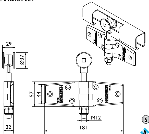
HANGROL 62K
