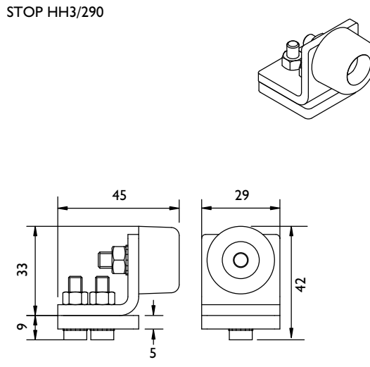
STOP HH3/290
