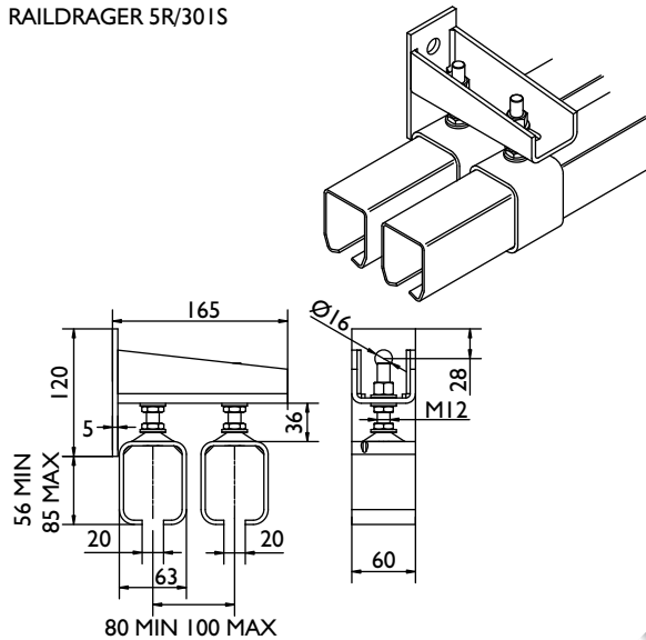
RAILDRAGER 5R/30IS
