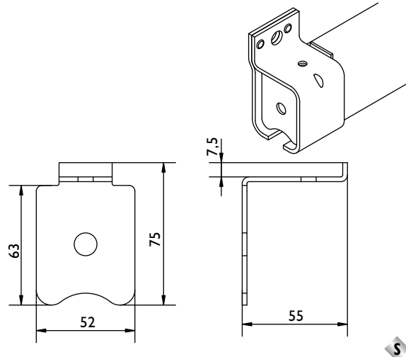
EINDCLIP 1A/30IEC
