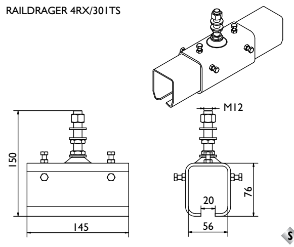
RAILDRAGER 4RX/30ITS
