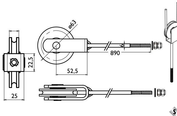
KATROL B-905
