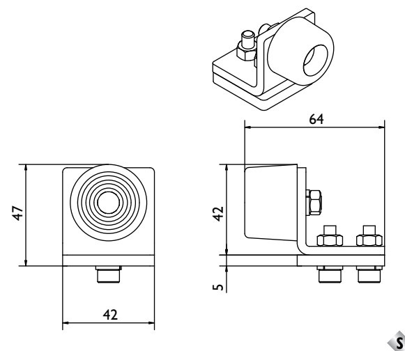
STOP HH3/30I
