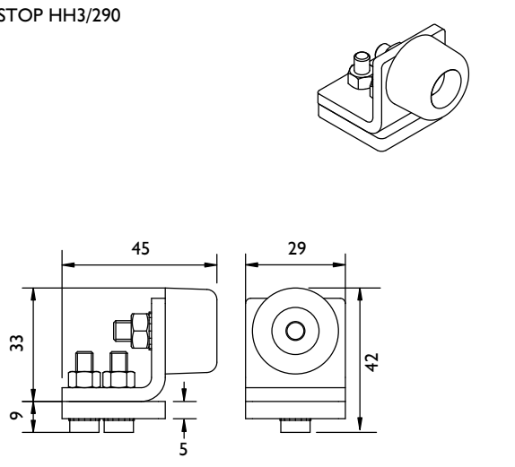
STOP HH3/290
