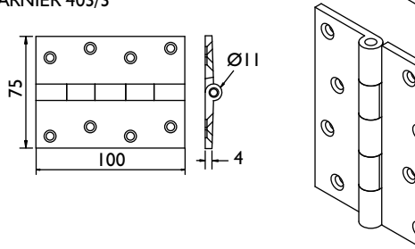
SCHARNIER 403/3
